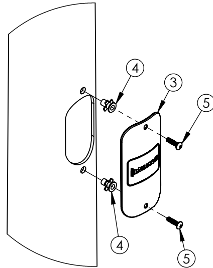
DETAIL A COVER ASSEMBLY SCALE 1 : 6
