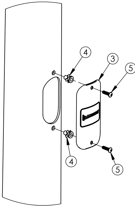
DETAIL A COVER ASSEMBLY SCALE 1 : 6
