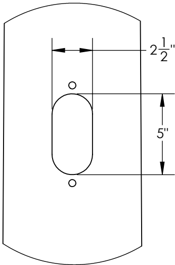
DETAIL B HANDHOLE CUTOUT COVER REMOVED FOR CLARITY SCALE 1 : 6
