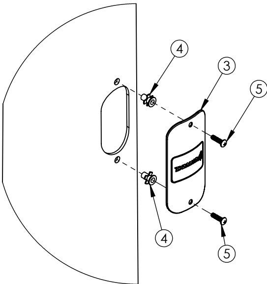
DETAIL A COVER ASSEMBLY SCALE 1:6
